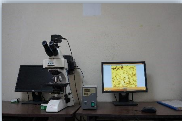
Fluorescence Spectroscopy
